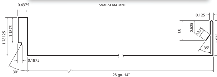
STRONGSEAM SSZSL175 PANEL SNAP-SEAM PANEL
