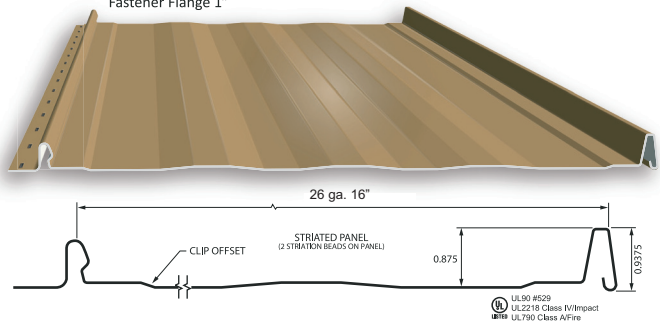
STRONGSEAM SSFF1 PANEL Fastener Flange 1"
