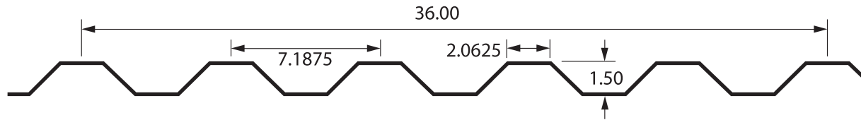
7.2 Roof Panel
