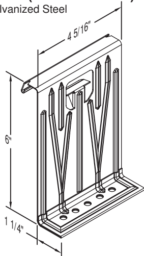
Part No. FC609 Weight - 0.446
