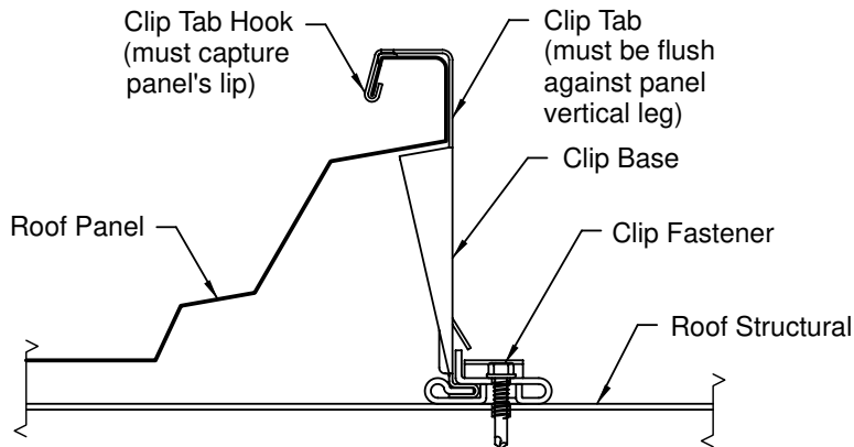
CLIP / PANEL ASSEMBLY
