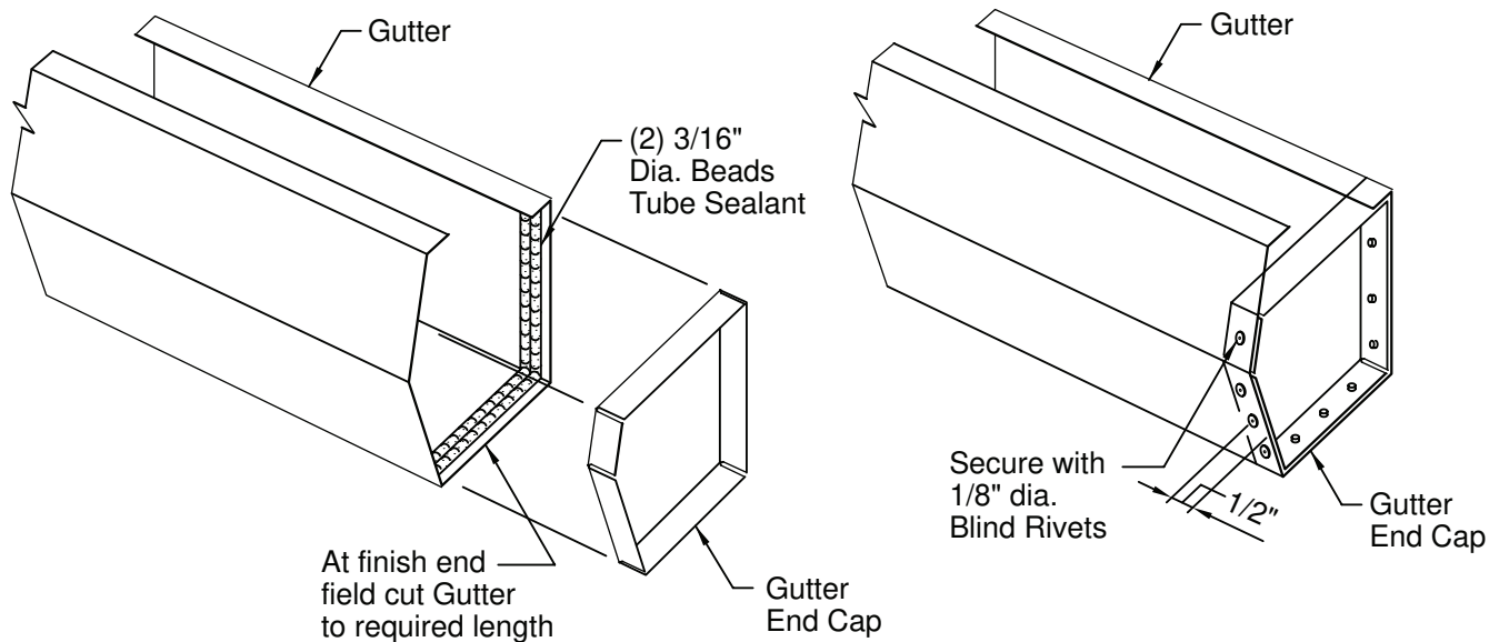
EAVE GUTTER END CAP
