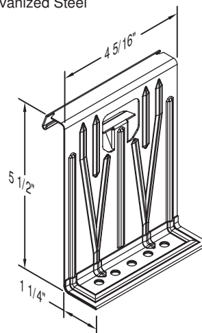
Part No. FC608 Weight - 0.423
